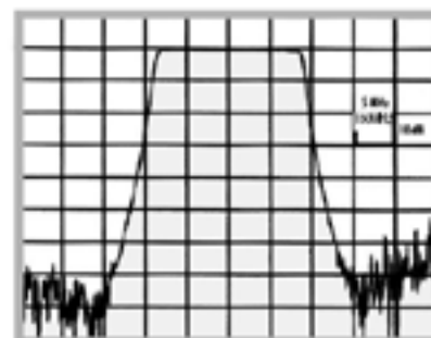
Typical Response Curve of 13961
